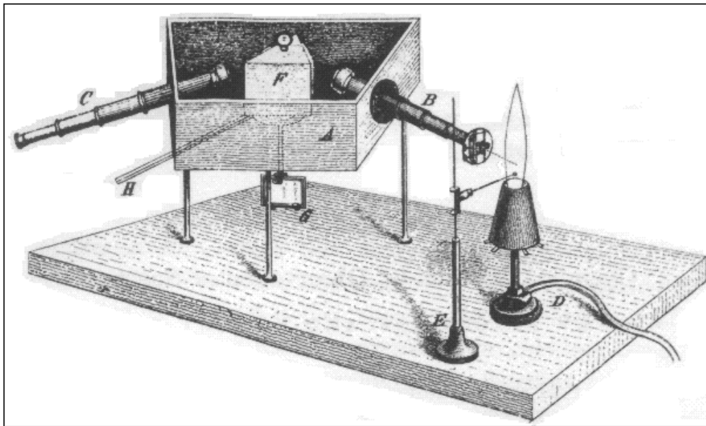
Spectroscope (1860)
